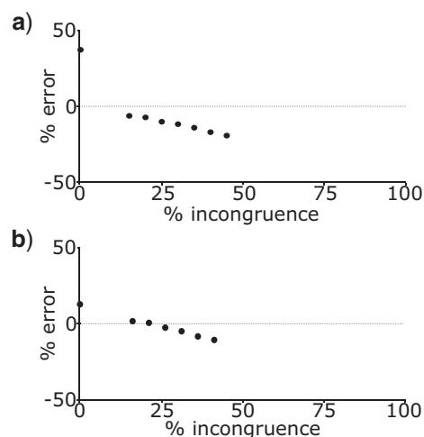
FIGURE 8. Percentage error of mean posterior estimates of t for branches in the species tree, plotted against the percentage of gene trees that are topologically incongruent for that branch, when analyzing data from the multispecies coalescent 16 taxon simulations. These plots summarize results across 50 replicated experiments when all simulated data is analyzed. The black points represent the mean percentage error in estimates of t for a given level of topological incongruence, with topological incongruence in bins of 5%. a) refers to the balanced species tree and b) refers to the imbalanced species tree.
